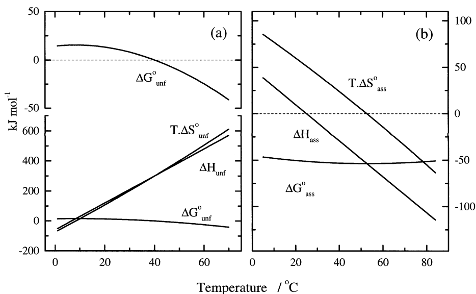
Fig. 3. Typical thermodynamic parameters as a function of temperature for biomolecular processes determined by microcalorimetry. (a) Free energy ( \Delta G^\circ_{\text{unf}} ), enthalpy ( \Delta H^\circ_{\text{unf}} ) and entropy ( T\Delta S^\circ_{\text{unf}} ) of unfolding in solution of a typical globular protein, with heat capacity increment upon infolding, \Delta C_p = 9 \text{ kJ K}^{-1} \text{ mol}^{-1} . The free energy data are also shown expanded in the upper panel, for clarity. (b) Free energy ( \Delta G^\circ_{\text{ass}} ), enthalpy ( \Delta H^\circ_{\text{ass}} ) and entropy ( T\Delta S^\circ_{\text{ass}} ) of association interaction between protein subunits in solution. In this case the strong temperature dependence of the enthalpy (heat) of binding corresponds to a \Delta C_p value of -1.9 \text{ kJ K}^{-1} \text{ mol}^{-1} , typical of many such interactions [10–12], and shows how the enthalpy may even change sign, being endothermic at low temperatures but exothermic at higher temperatures.
